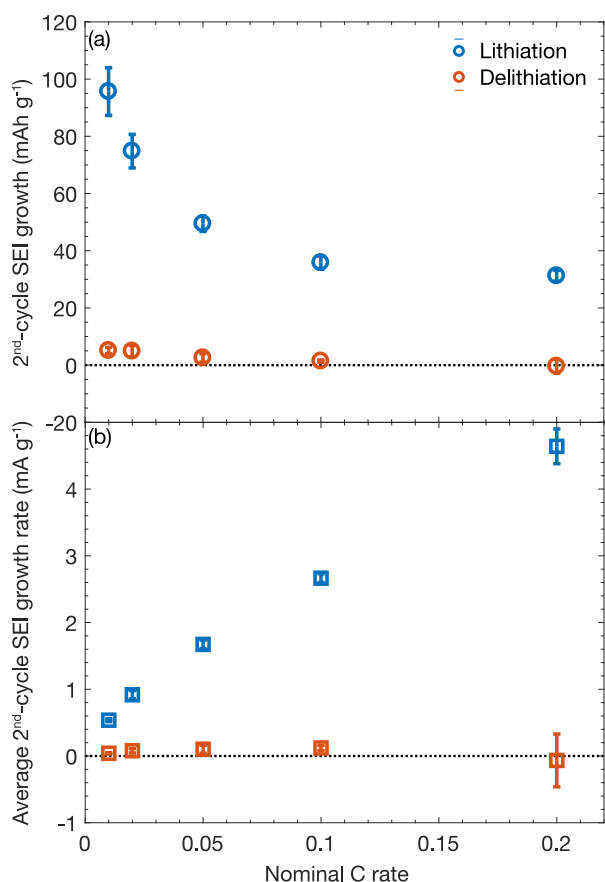
Figure 6. Second-cycle SEI growth as a function of current magnitude and current direction, averaged over three cells. (a) Dependence of second-cycle SEI growth on nominal C rate. These capacities are calculated from the integral of the \Delta dQ/dV curves in Figure 5. (b) Dependence of second-cycle average SEI growth rate on nominal C rate. The average SEI growth rate (units of mA g -1 ) is calculated by dividing the SEI capacity (mAh g -1 ) by the time per cycle (h). A linear fit of the lithiation data to nominal applied current yields the equation y = (0.11 \pm 0.01)x + (0.5 \pm 0.3 \text{ mA g}^{-1}) , where errors represent the 95% CI. In both subplots, the error bars represent 95% confidence intervals of the mean.
